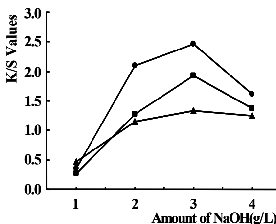
Fig. 1. K/S values of silk(●), cotten(■), and yam(▲) with polygoum tinctoria dyes as a function of various sodium hydroxide concentration.
