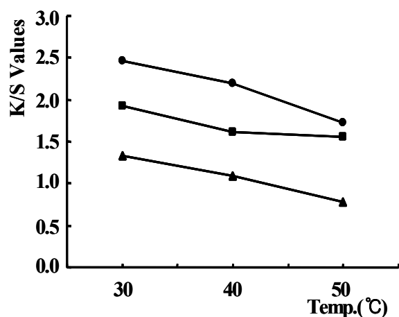
Fig. 3. K/S values of silk(●), cotton(■), and yam(▲) with polygoum tinctoria dyes as a function of various dyeing temperature
