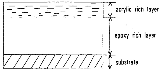
Fig. 6 Film model of epoxy-acrylic ED resin
