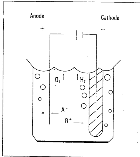
Fig. 4 Schematic diagram of the cathodic electro-deposition process
