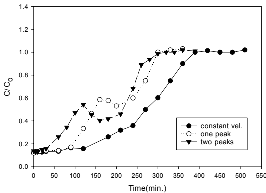
Fig. 3 Effect of one and two peaks in velocity on silica breakthrough curve.
