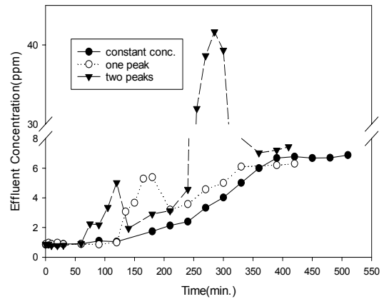
Fig. 2 Effect of one and two peaks in feed concentration on silica breakthrough curve.
