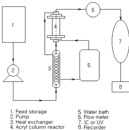
Fig. 1 Schematic diagram of continuous experimental system.
