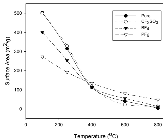
Figure 2. The effect of anion parts in ionic liquid with [Bmim + ] on surface area of TiO_2 particles obtained with heat treatment at various temperatures.
