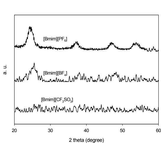
Figure 1. XRD patterns of TiO_2 particles prepared using various ionic liquids with heat treatment at 100^\circ C .
