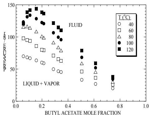
Figure 1. Pressure-composition experimental data of Carbon dioxide-butyl acetate system.
