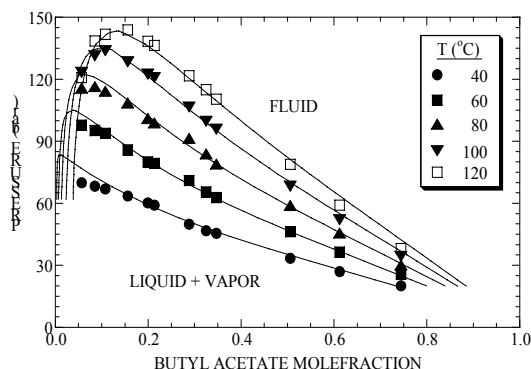
Figure 4. Comparison of the experimental data for the carbon dioxide-butyl acetate system with calculated values obtained with Peng-Robinson equation of state
