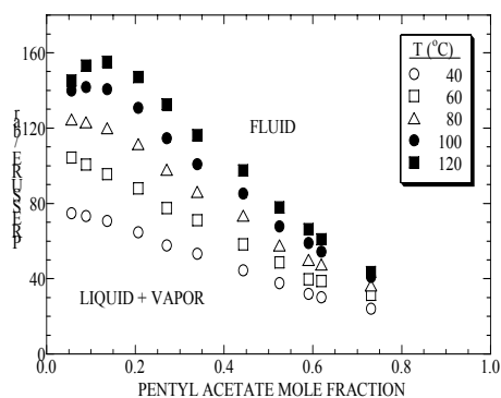
Figure 2. The phase behavior data of carbon dioxide-pentyl acetate system.
